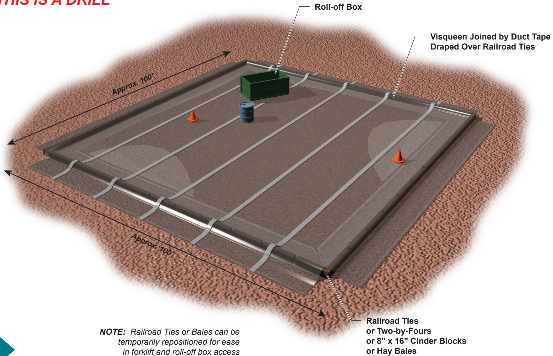
SCHEMATIC DRAWING OF WASTE STAGING AREA
